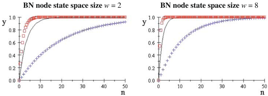
Fig. 1 The probability of a randomly picked BN explanation x being zero, or y = \Pr(U_M(x) = 0) , as a function of varying BN size n (along the x -axis), CPT entry zero probability \rho , and BN node state space size w . The curves are for varying \rho , with \rho = 0.1 (curve indicated by blue crosses ), \rho = 0.5 (curve indicated by black line ), and \rho = 0.9 (curve indicated by red squares ). The BN node state space size is different in these two panels . Left panel : State space size w = 2 ; Right panel : State space size w = 8
